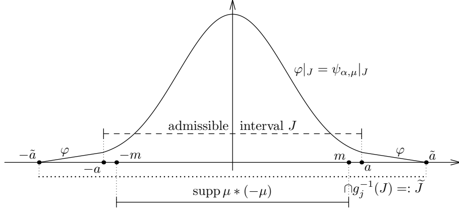
Figure 10: The construction of function \varphi in Lemma 5.12. It agrees with \psi_{\alpha,\mu} on the admissible interval J , is linear on \tilde{J} \setminus J and vanishes outside of \tilde{J} .
